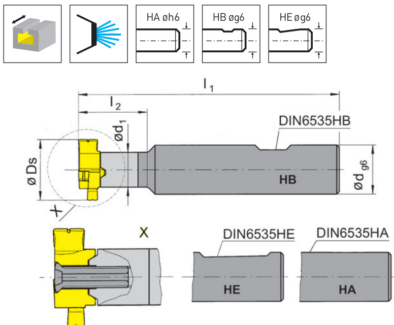
Abbildung = rechtsschneidend Picture = right hand cutting version
